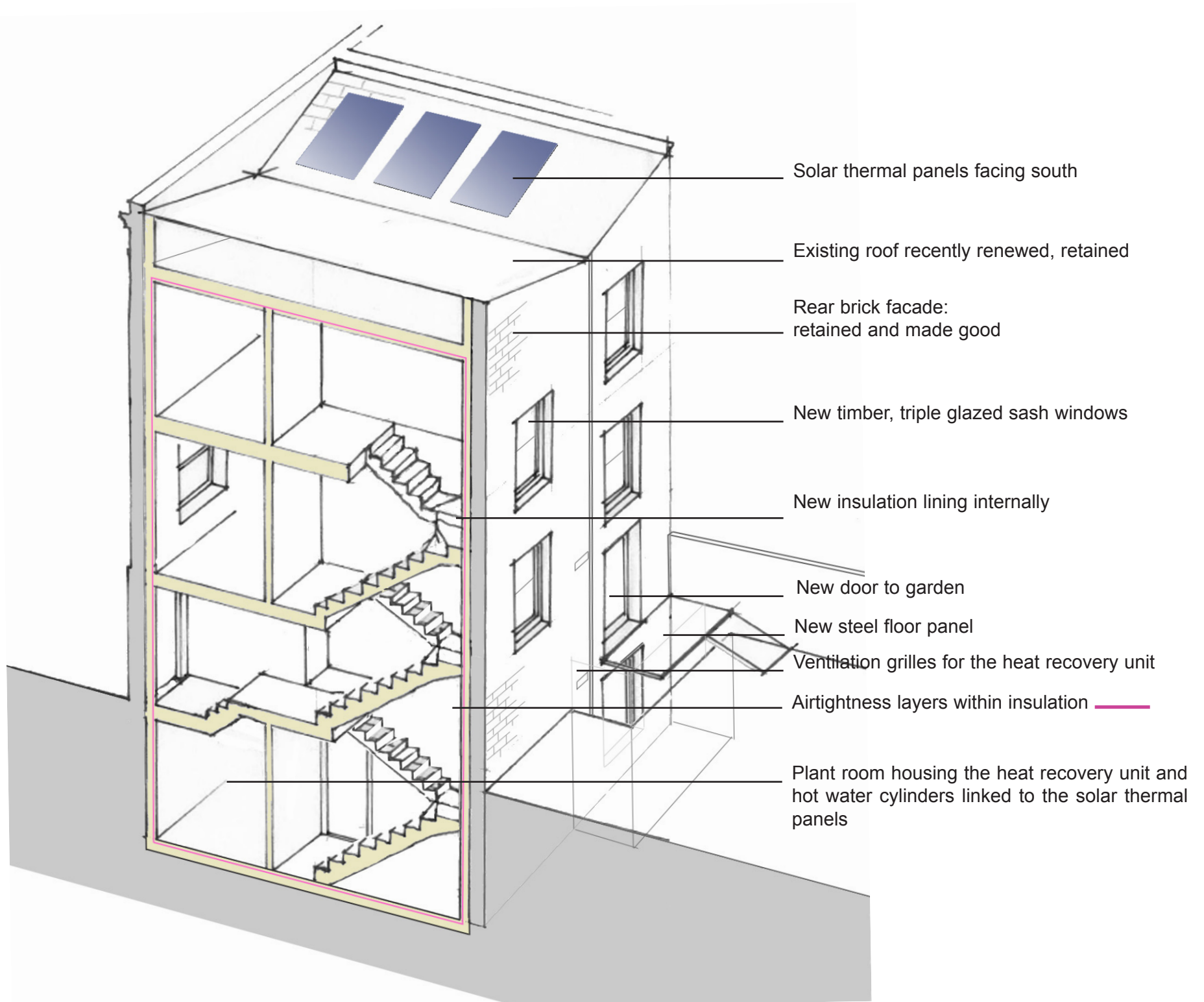
Perspective - Section illustrating the environmental principles
