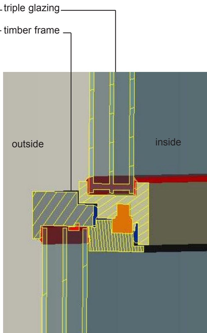
Detail of proposed sash window transom
